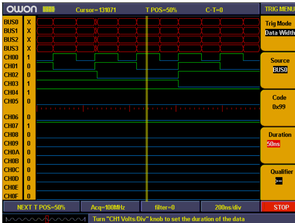
Fig 73: Data width trigger
