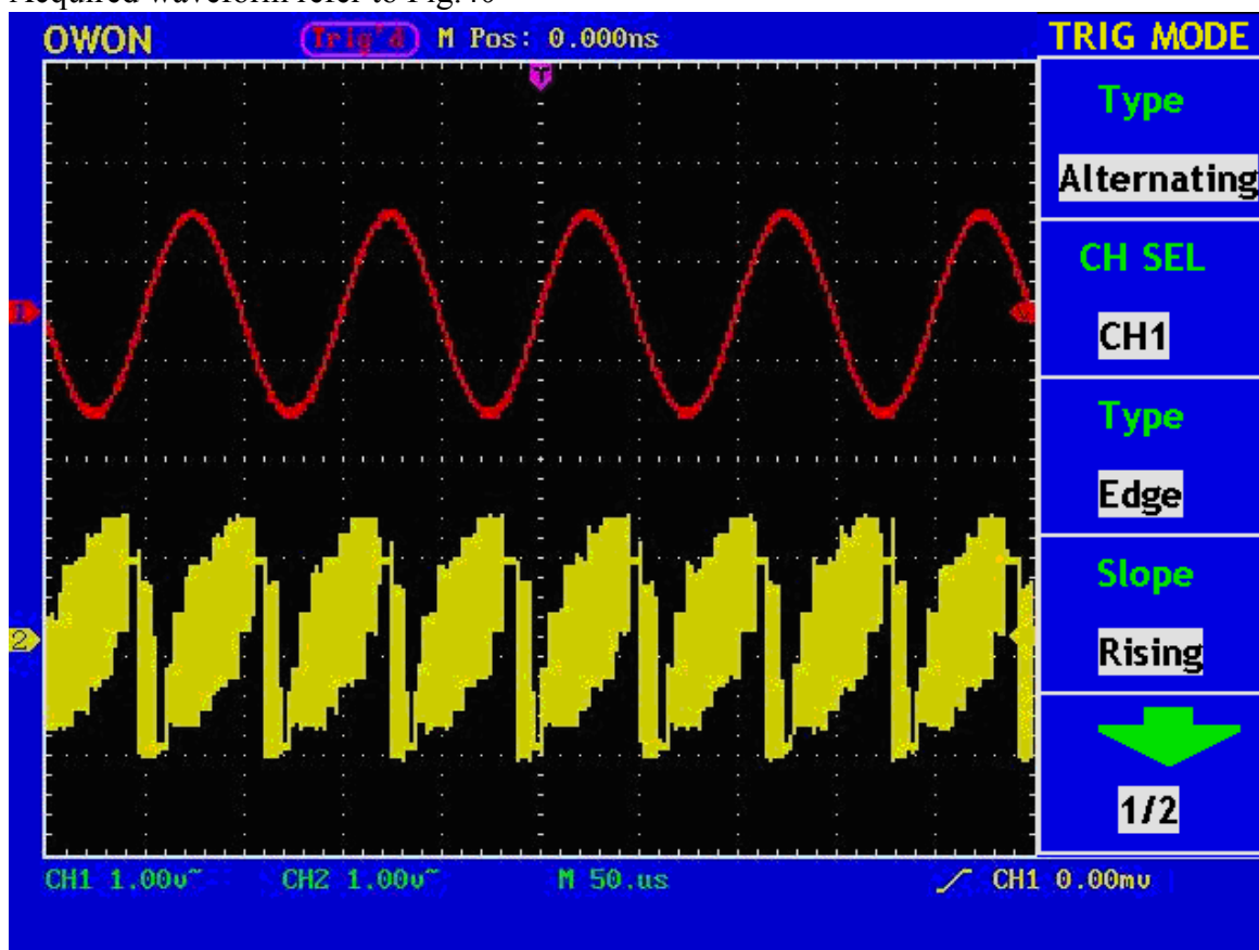
Fig. 40 Alternate trigger Oscillogram
